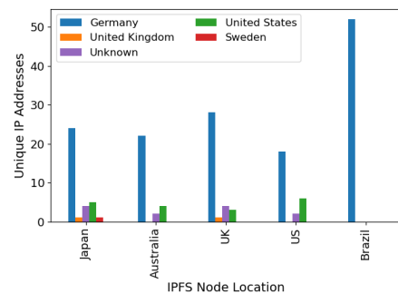
Fig. 4: All IP Geo-location for peers downloaded decoy files with respect to each deployed IPFS node.
